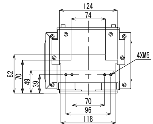
Positions of Screws for Extension Guide 延長ガイド用ねじ位置
