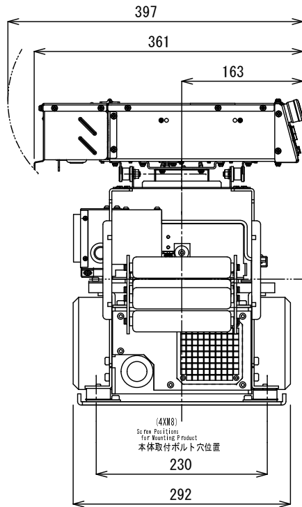
Overall Dimensions Drawing of Model TG4
